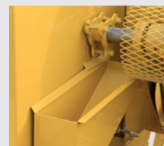
Internally lubricated packing gland with drip catch pan
